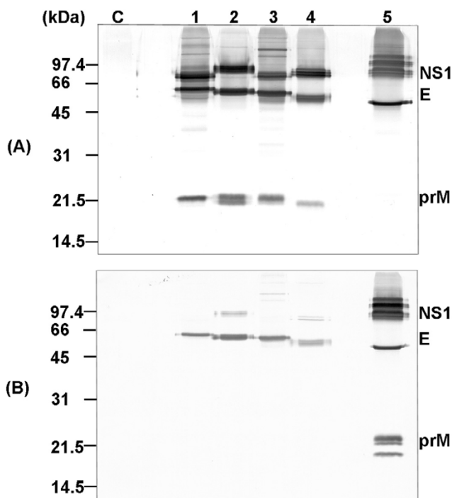
Figure 1 Immunoblots Probed With High Titled Antiserum Pools. SDS PAGE was run with samples which were not reduced with 2-mercaptoethanol and not heated before electrotransfer to nitrocellulose membranes. Immunoblots were probed with (A): convalescent dengue serum (HPR) and (B): JEV positive swine serum (PPJ). Lane C contains uninfected cell lysates while Lanes 1, 2, 3, 4 and 5 contain lysates of DENV1, 2, 3, 4 and JEV respectively. The position for bands of NS1 dimer, E and prM are labeled on the right.
